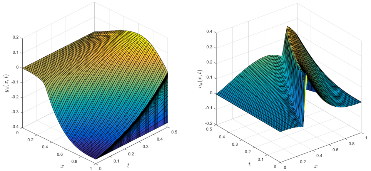
Figure 2: Surface plot of numerical approximation to y and u with \varepsilon = 2^{-12} and N = M = 64 for Example 5.2.
